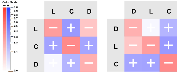
Figure 4: The \phi matrix considering only the three main categories for all the data across languages. In the left figure, the categories are sorted according to their position in the oral cavity. In the right figure, the categories are sorted automatically, which shows that D and L are more similar to each other than D and C .
